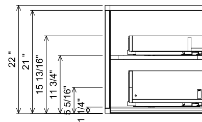
AT SINK CENTER SECTION
