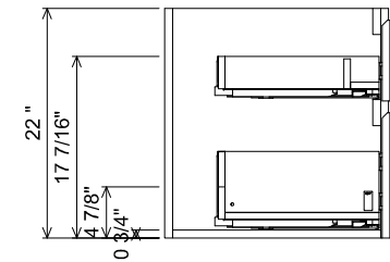
AT SINK CENTER SECTION
