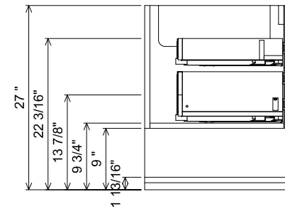
AT SINK CENTER SECTION
