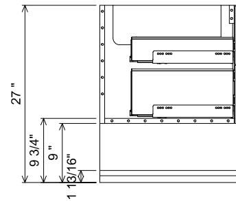
AT BANK SECTION
