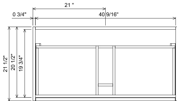
BENEATH BRACE
