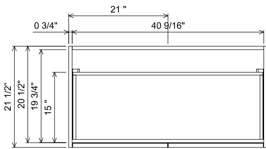
AT BOTTOM DRAWER SECTION
