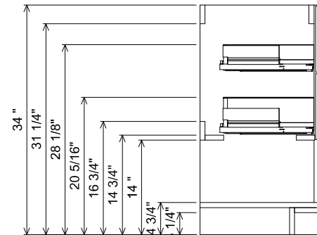
AT SINK CENTER SECTION
