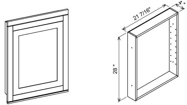
RECESSED CABINET MEASUREMENTS
