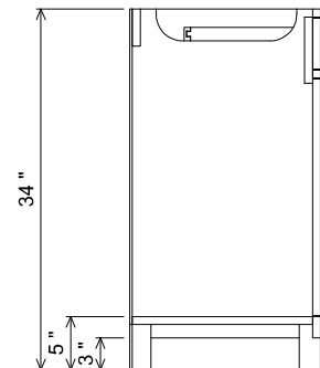
AT SINK CENTER SECTION
