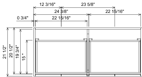
AT BOTTOM DRAWER SECTION 1:20
