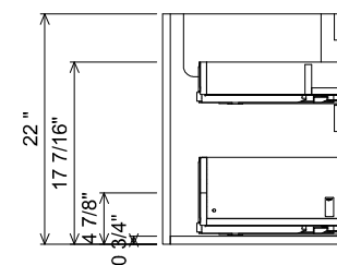
AT SINK CENTER SECTION
