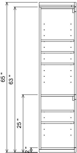
SECTION
