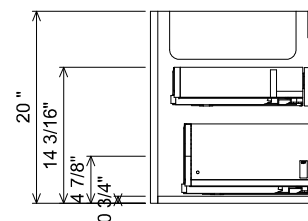
AT CENTER SINK SECTION
