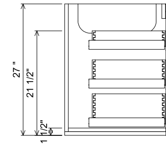
AT BANK SECTION
