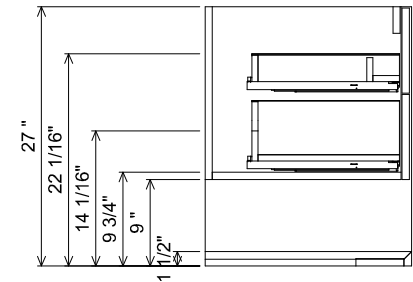
AT SINK CENTER SECTION
