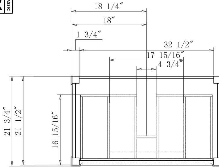
TRIM DETAIL
