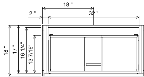
AT BENEATH BRACE SECTION
