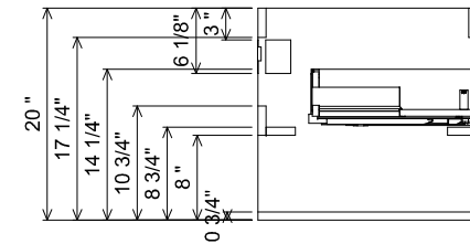
AT SINK CENTER SECTION
