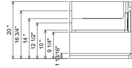
AT SINK CENTER SECTION
