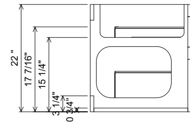
AT SINK CENTER SECTION
