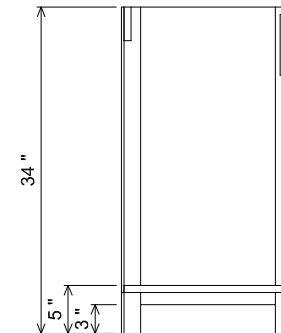
AT SINK CENTER SECTION
