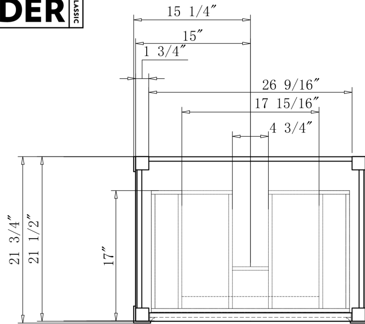
TRIM DETAIL
