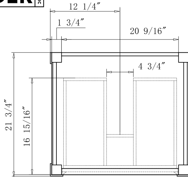
TRIM DETAIL
