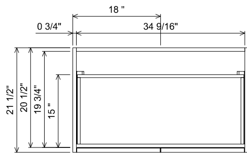
AT BOTTOM DRAWER SECTION
