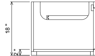
AT SINK CENTER SECTION
