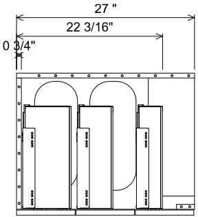
AT BANK SECTION
