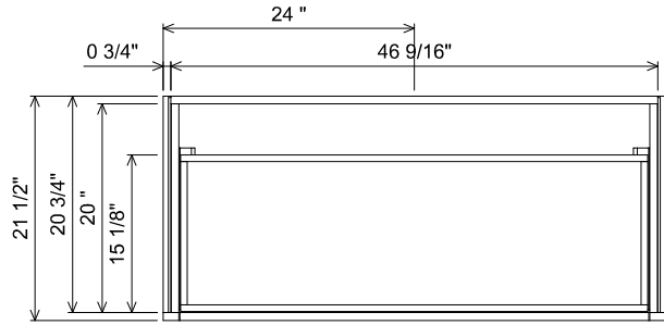
AT BOTTOM DRAWER SECTION
