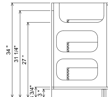
AT BLIND CENTER SECTION
