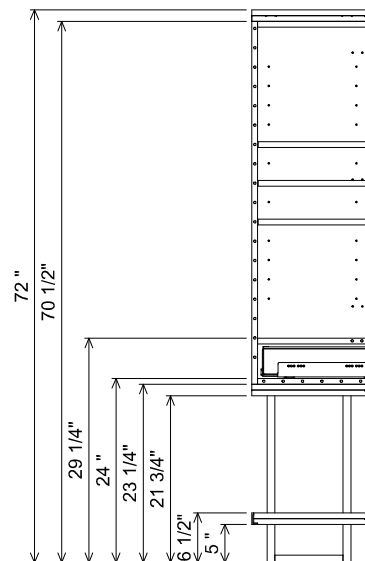
SECTION
