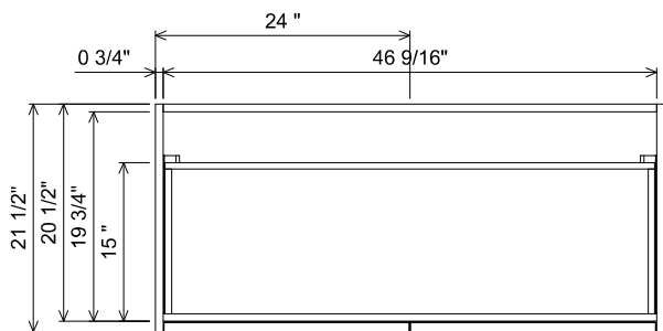
AT BOTTOM DRAWER SECTION
