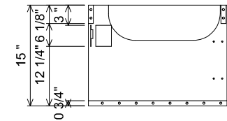
AT WING SECTION
