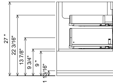
AT SINK CENTER SECTION
