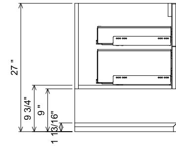
AT BANK SECTION
